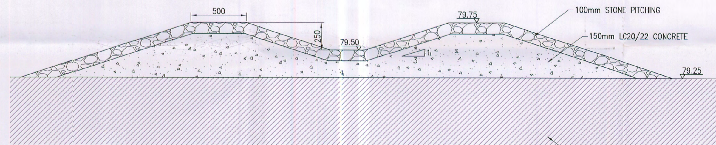
SECTION E-E
